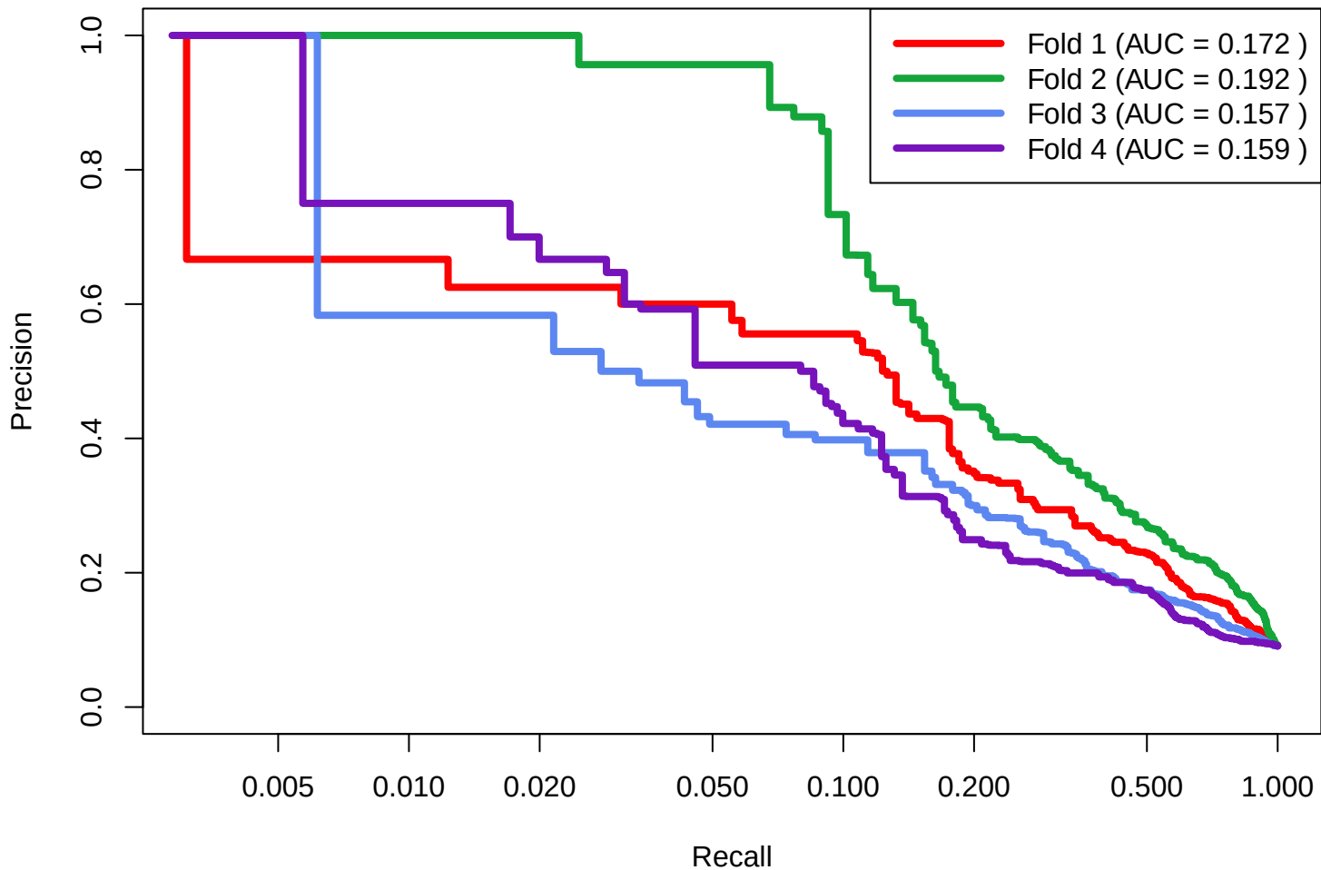
SPELL Original Datasets: 0.50 Training
